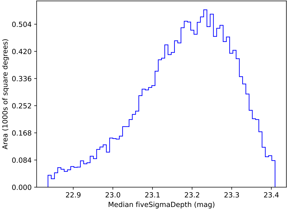
ddf_loaded_fl2_v3.4_10yrs WFD u band: Median fiveSigmaDepth
