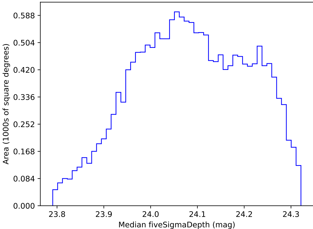
ddf_loaded_fl2_v3.4_10yrs WFD r band: Median fiveSigmaDepth
