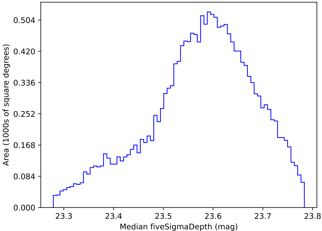
ddf_loaded_fl2_v3.4_10yrs WFD i band: Median fiveSigmaDepth
