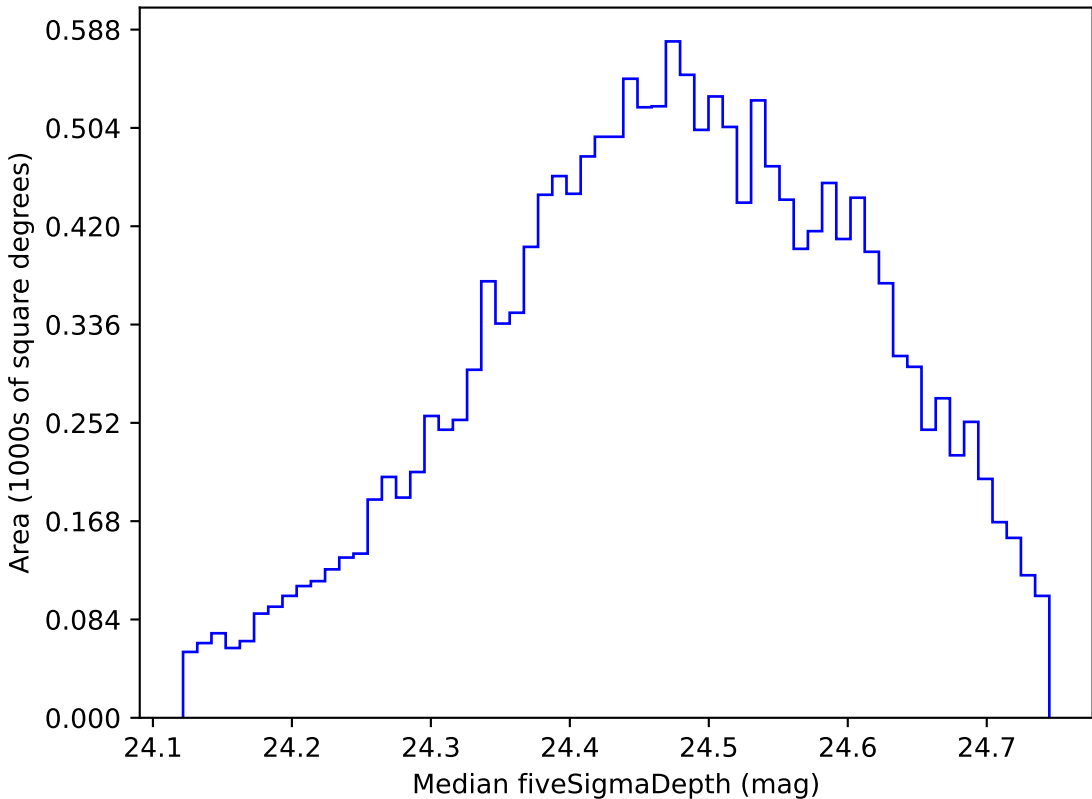
ddf_loaded_fl2_v3.4_10yrs WFD g band: Median fiveSigmaDepth
