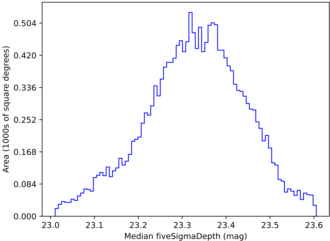
ddf_loaded_fl2_v3.4_10yrs WFD all bands: Median fiveSigmaDepth
