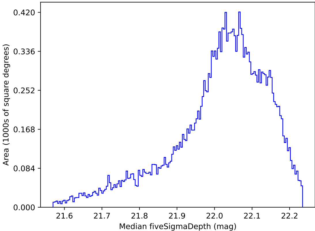
ddf_loaded_fl2_v3.4_10yrs All sky y band: Median fiveSigmaDepth
