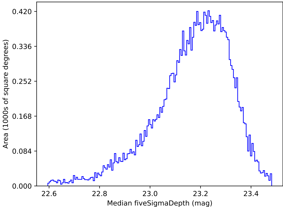
ddf_loaded_fl2_v3.4_10yrs All sky u band: Median fiveSigmaDepth
