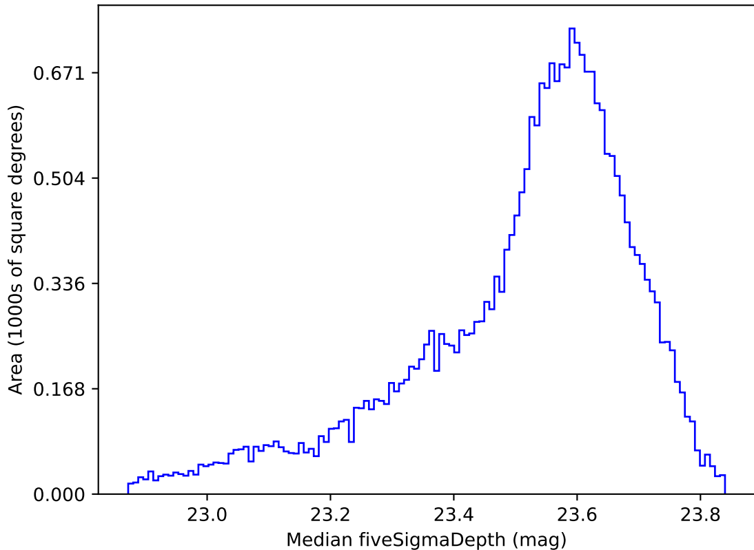
ddf_loaded_fl2_v3.4_10yrs All sky i band: Median fiveSigmaDepth
