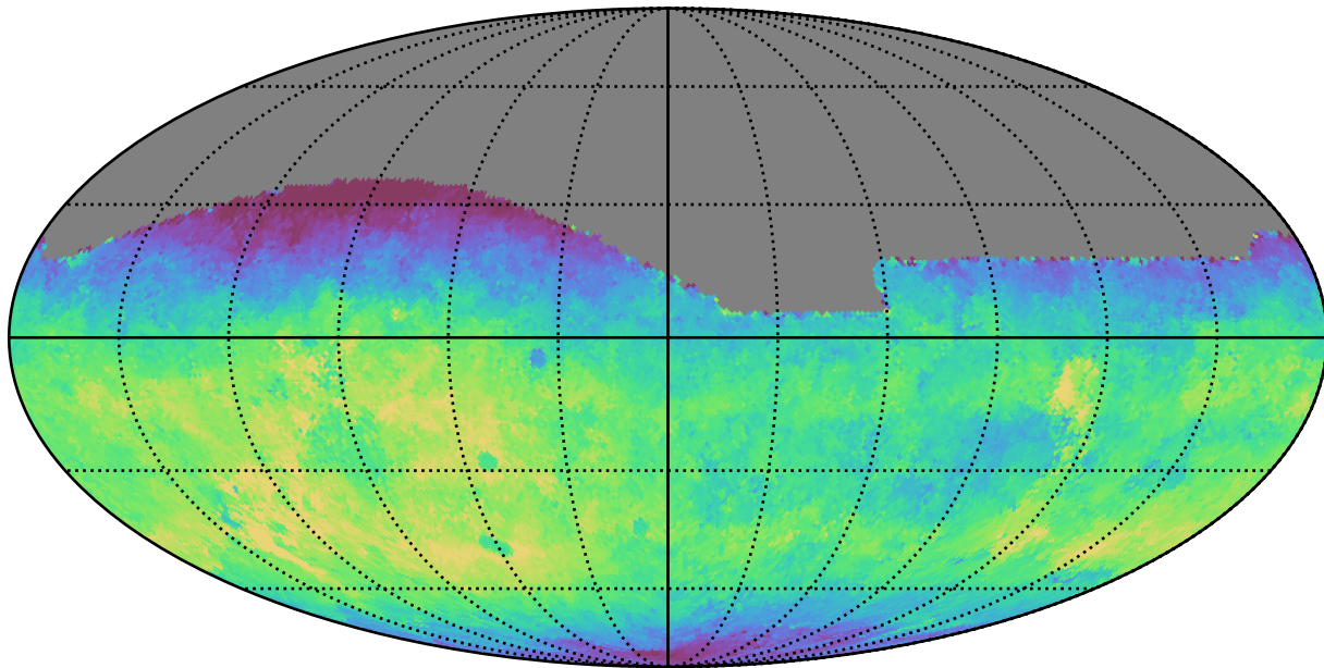
ddf_loaded_fl2_v3.4_10yrs All sky g band: Median fiveSigmaDepth
