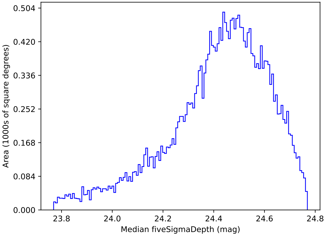
ddf_loaded_fl2_v3.4_10yrs All sky g band: Median fiveSigmaDepth
