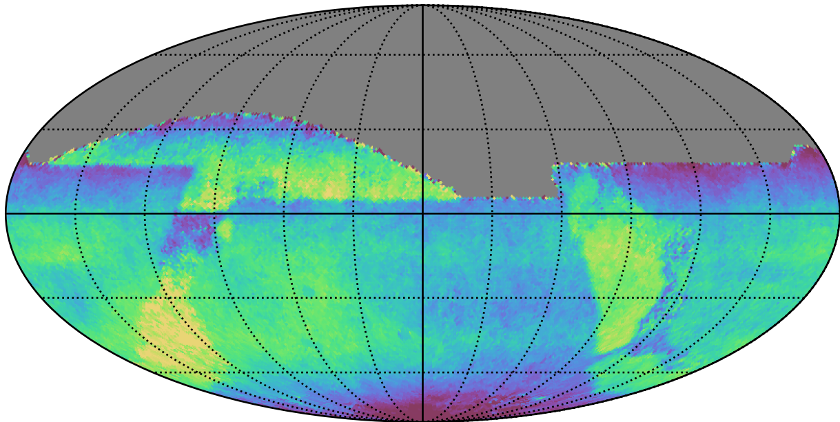
ddf_loaded_fl2_v3.4_10yrs All sky all bands: Median fiveSigmaDepth
