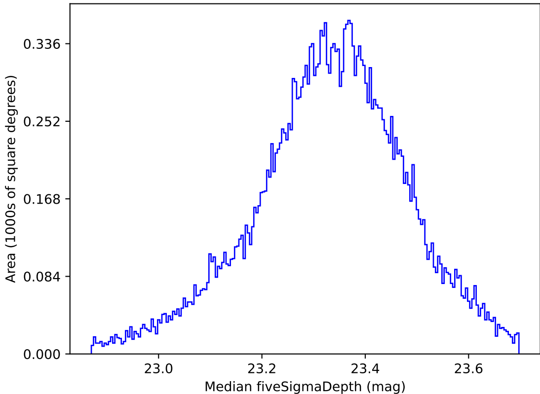
ddf_loaded_fl2_v3.4_10yrs All sky all bands: Median fiveSigmaDepth
