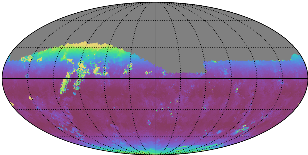
ddf_loaded_fl2_v3.4_10yrs Yr 1 z band: Median airmass
