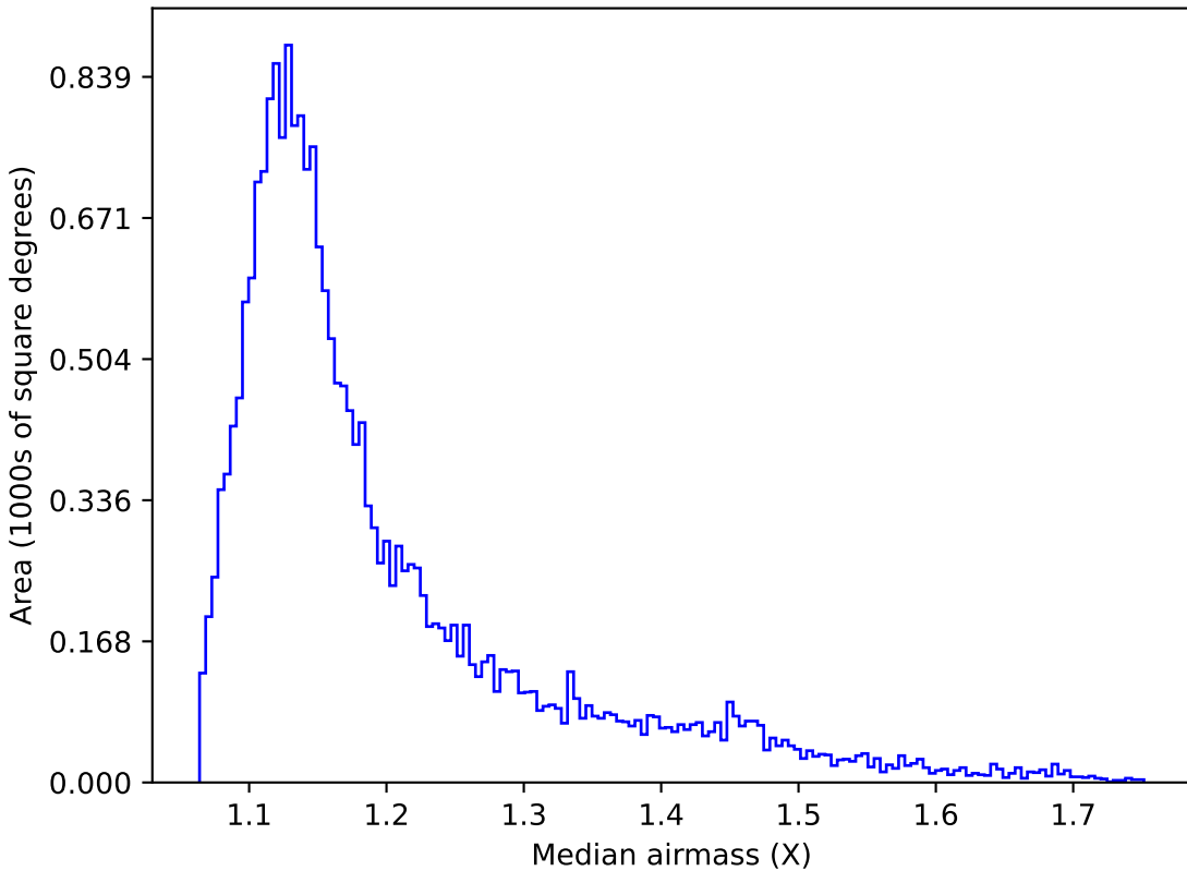
ddf_loaded_fl2_v3.4_10yrs Yr 1 y band: Median airmass
