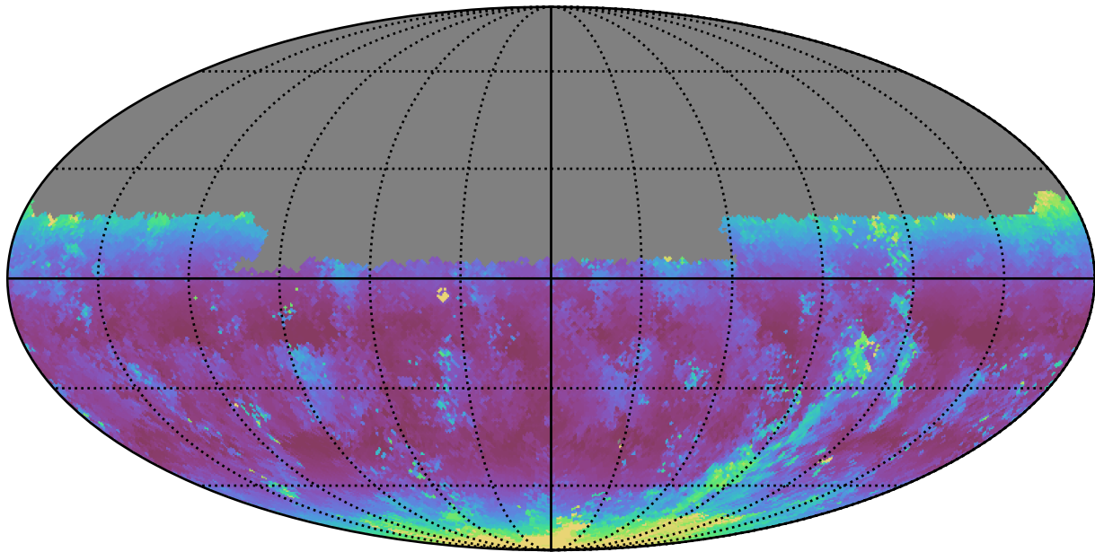
ddf_loaded_fl2_v3.4_10yrs Yr 1 u band: Median airmass
