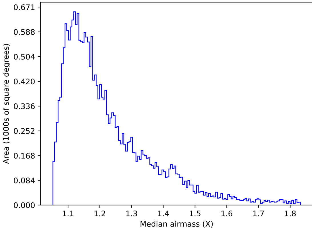
ddf_loaded_fl2_v3.4_10yrs Yr 1 u band: Median airmass
