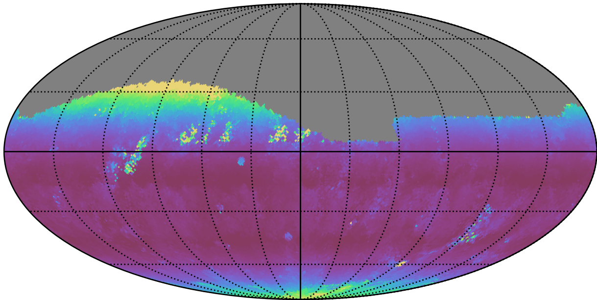
ddf_loaded_fl2_v3.4_10yrs Yr 1 r band: Median airmass
