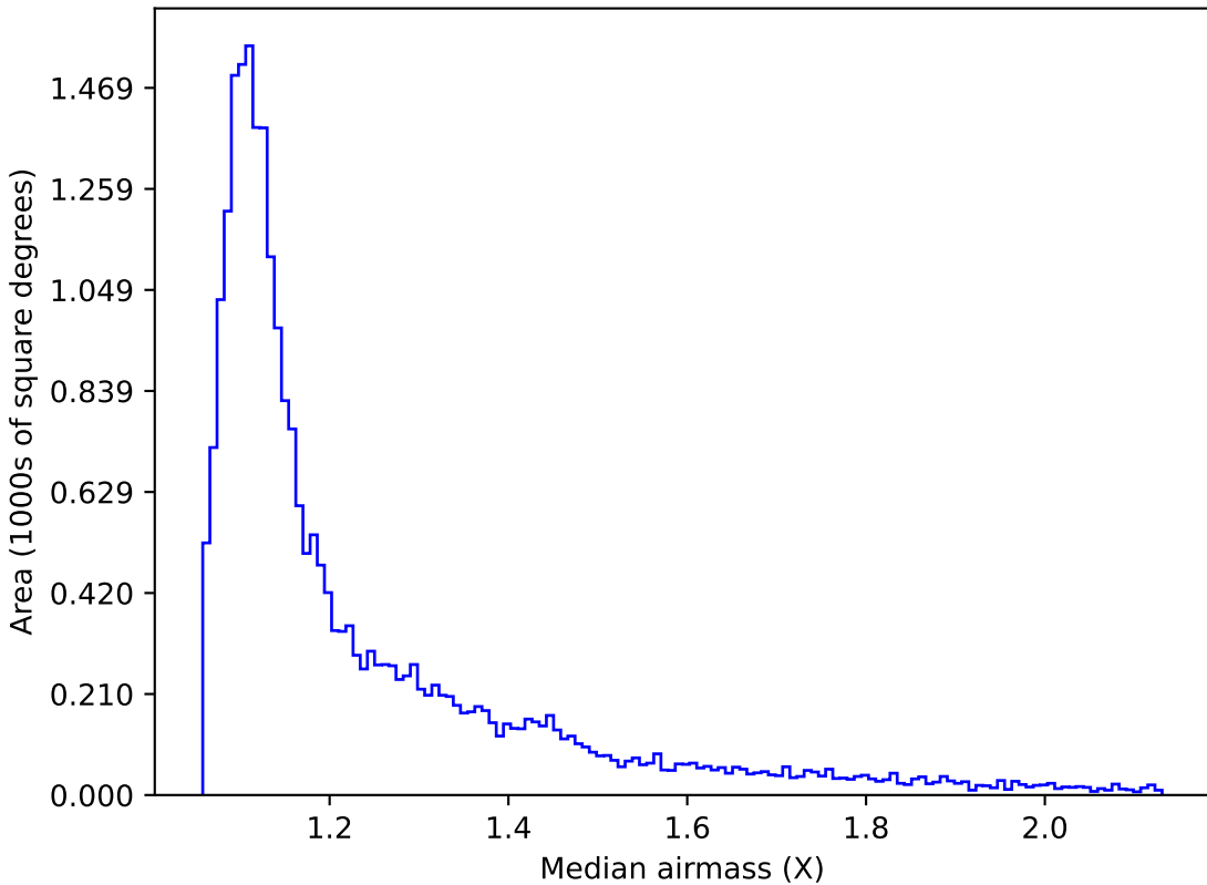
ddf_loaded_fl2_v3.4_10yrs Yr 1 r band: Median airmass
