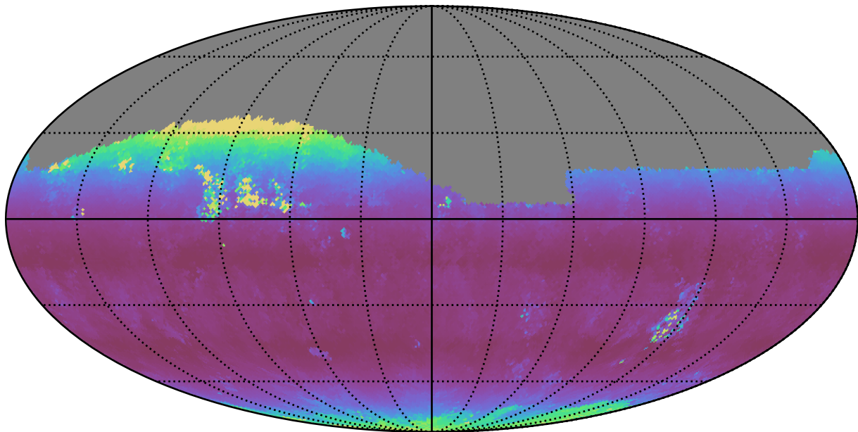
ddf_loaded_fl2_v3.4_10yrs Yr 1 i band: Median airmass
