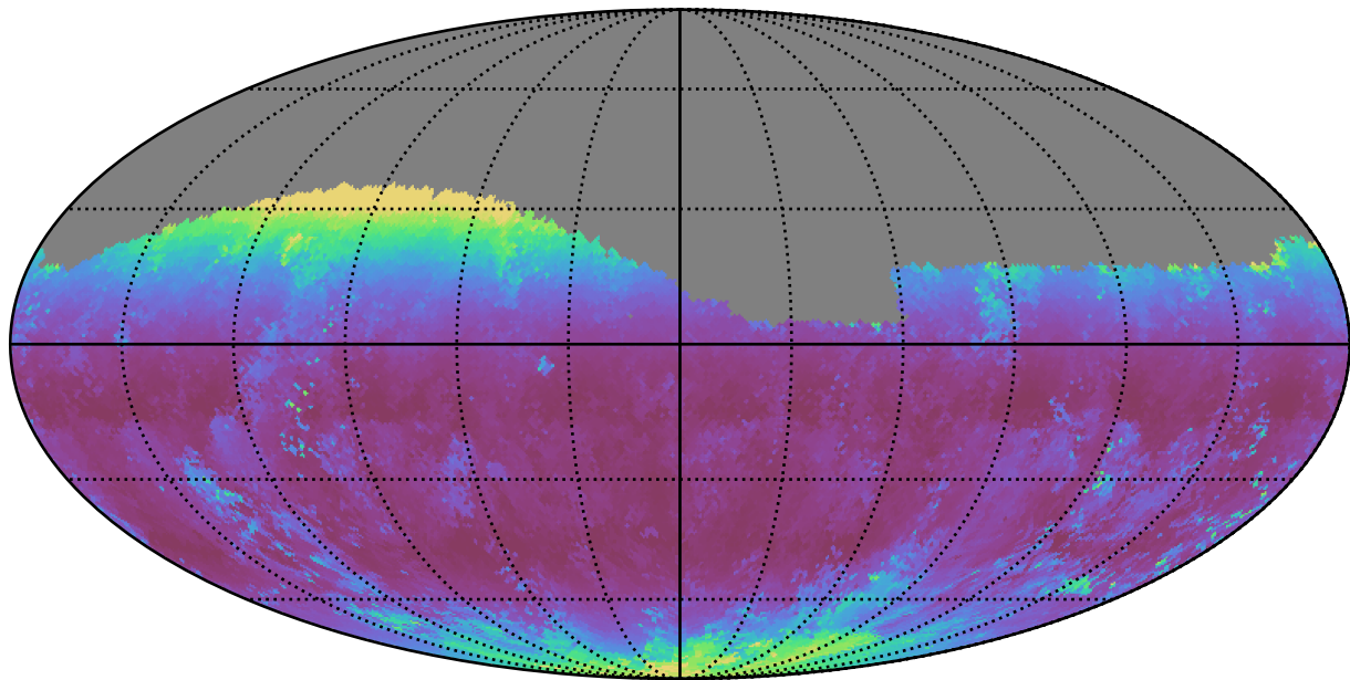
ddf_loaded_fl2_v3.4_10yrs Yr 1 g band: Median airmass
