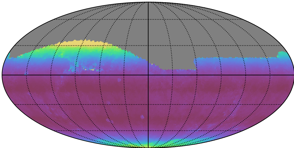
ddf_loaded_fl2_v3.4_10yrs Yr 1 all bands: Median airmass
