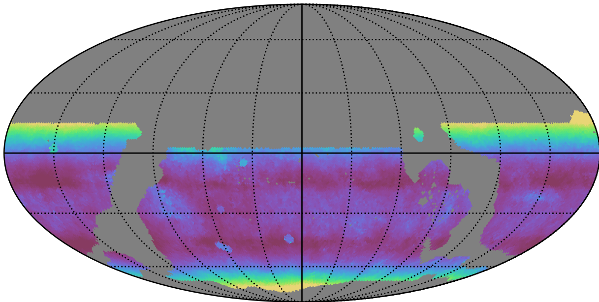
ddf_loaded_fl2_v3.4_10yrs WFD z band: Median airmass
