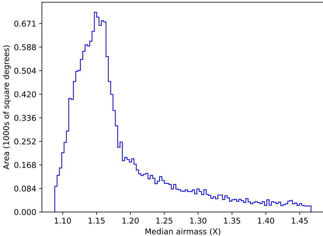
ddf_loaded_fl2_v3.4_10yrs WFD z band: Median airmass
