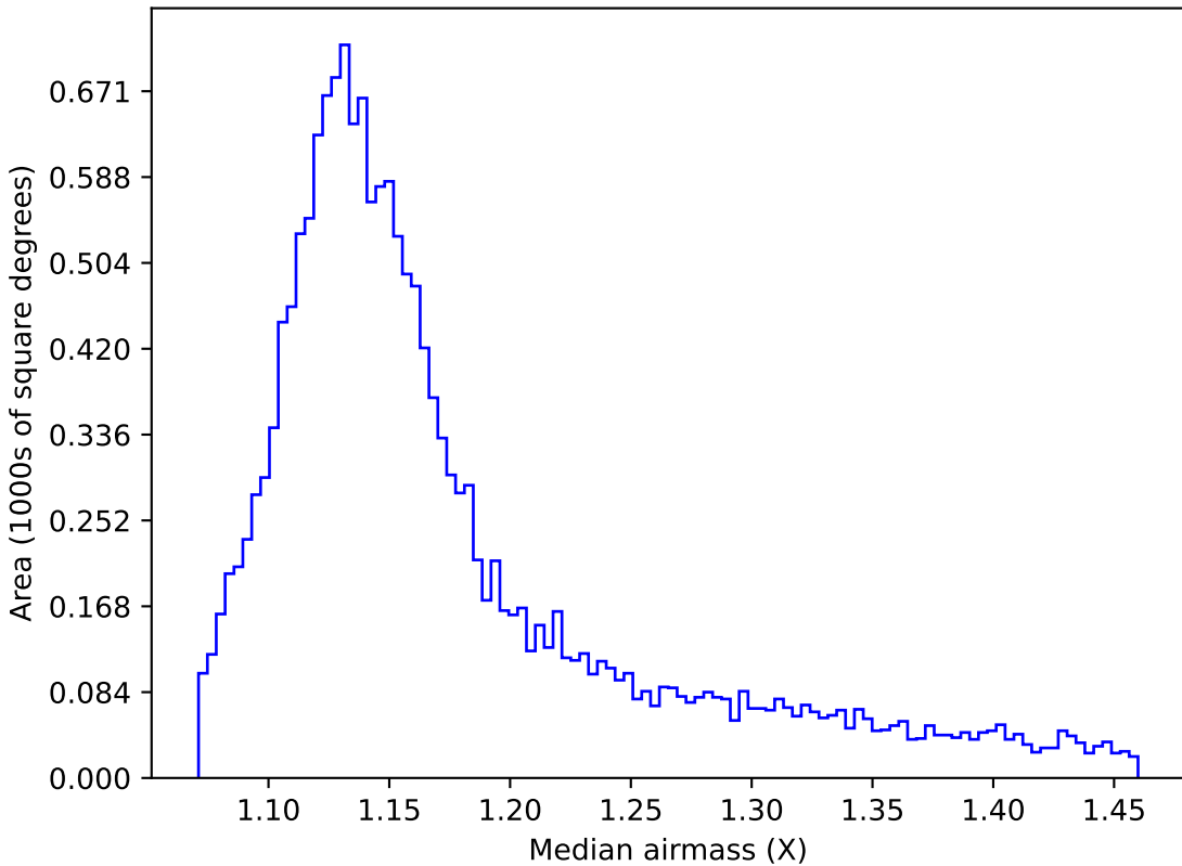
ddf_loaded_fl2_v3.4_10yrs WFD u band: Median airmass
