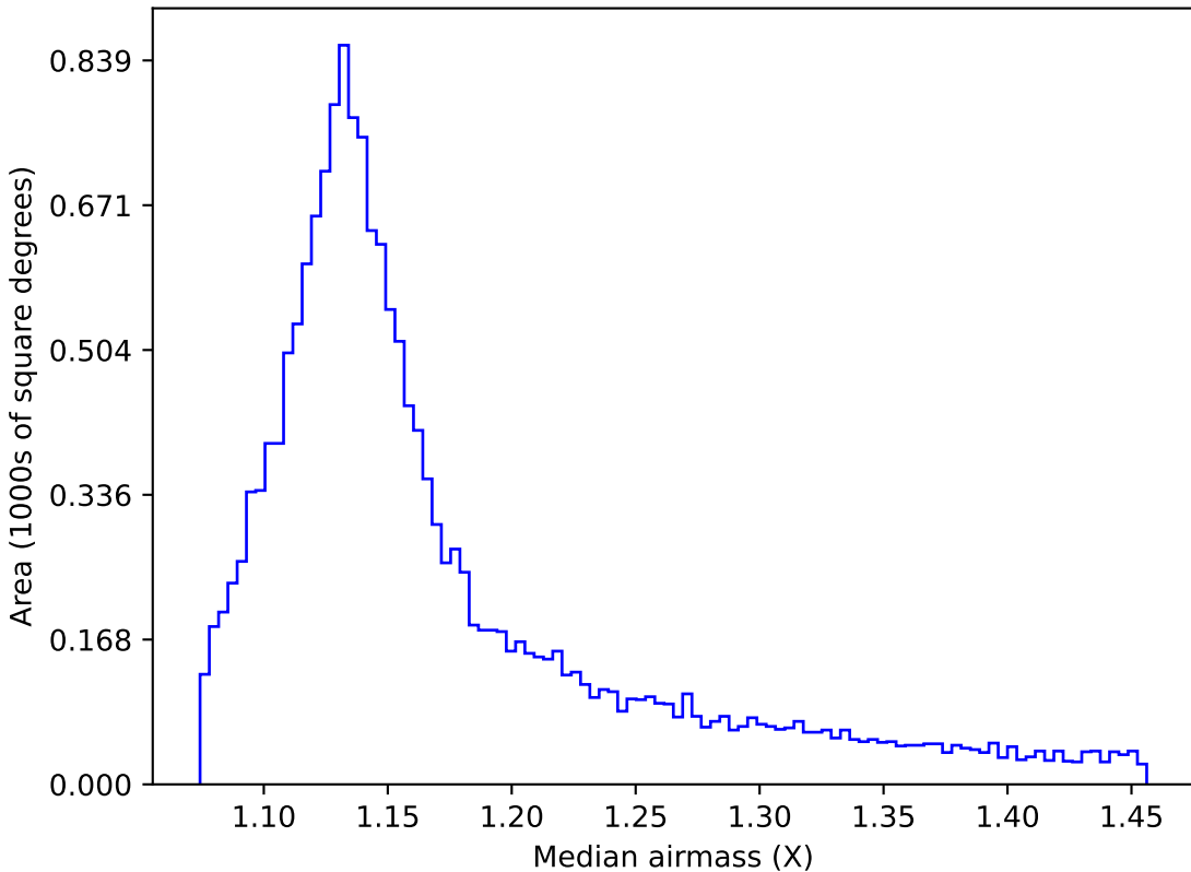
ddf_loaded_fl2_v3.4_10yrs WFD r band: Median airmass
