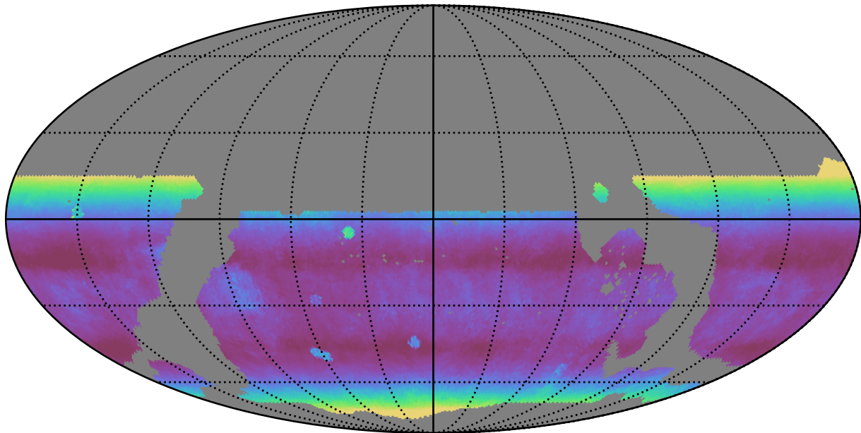
ddf_loaded_fl2_v3.4_10yrs WFD i band: Median airmass
