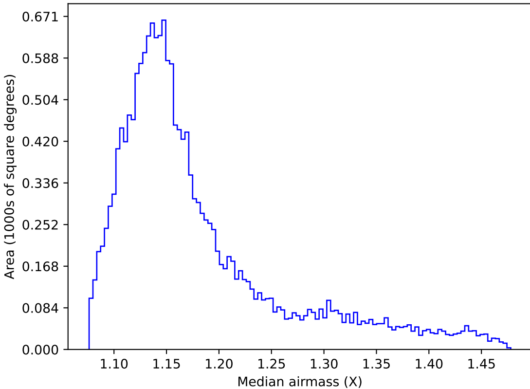
ddf_loaded_fl2_v3.4_10yrs WFD g band: Median airmass
