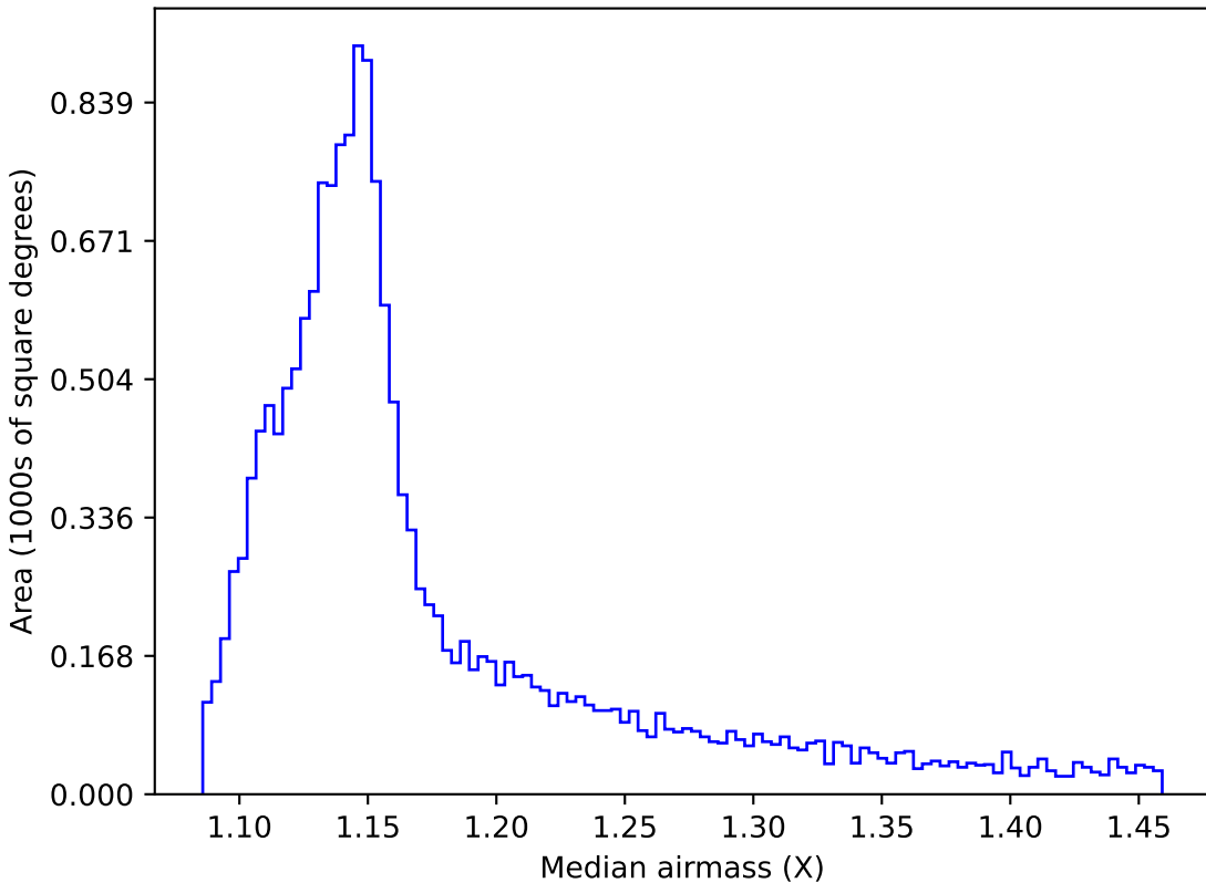
ddf_loaded_fl2_v3.4_10yrs WFD all bands: Median airmass
