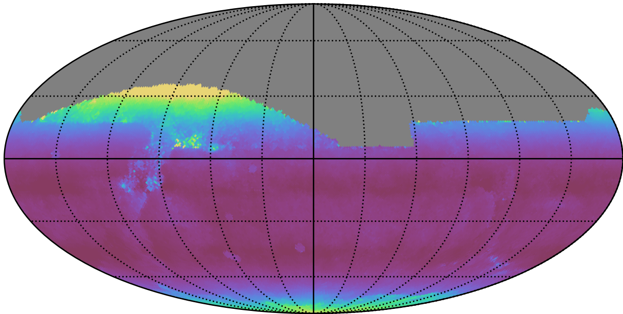
ddf_loaded_fl2_v3.4_10yrs All sky z band: Median airmass
