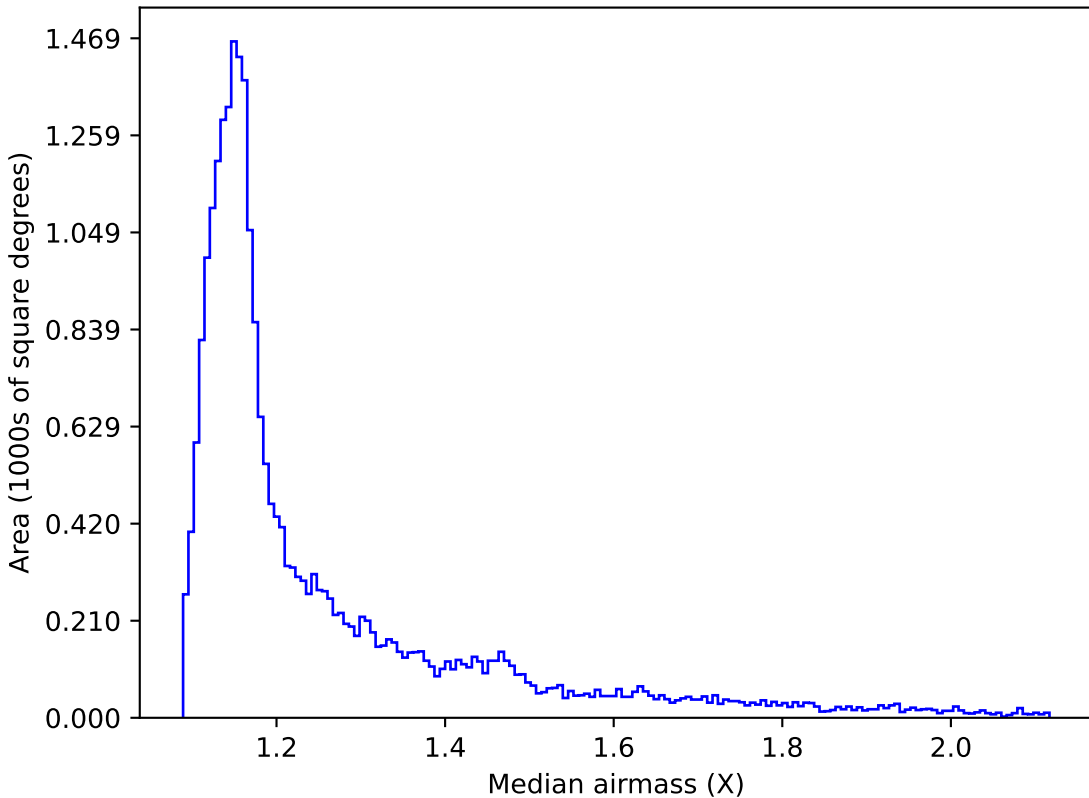
ddf_loaded_fl2_v3.4_10yrs All sky z band: Median airmass
