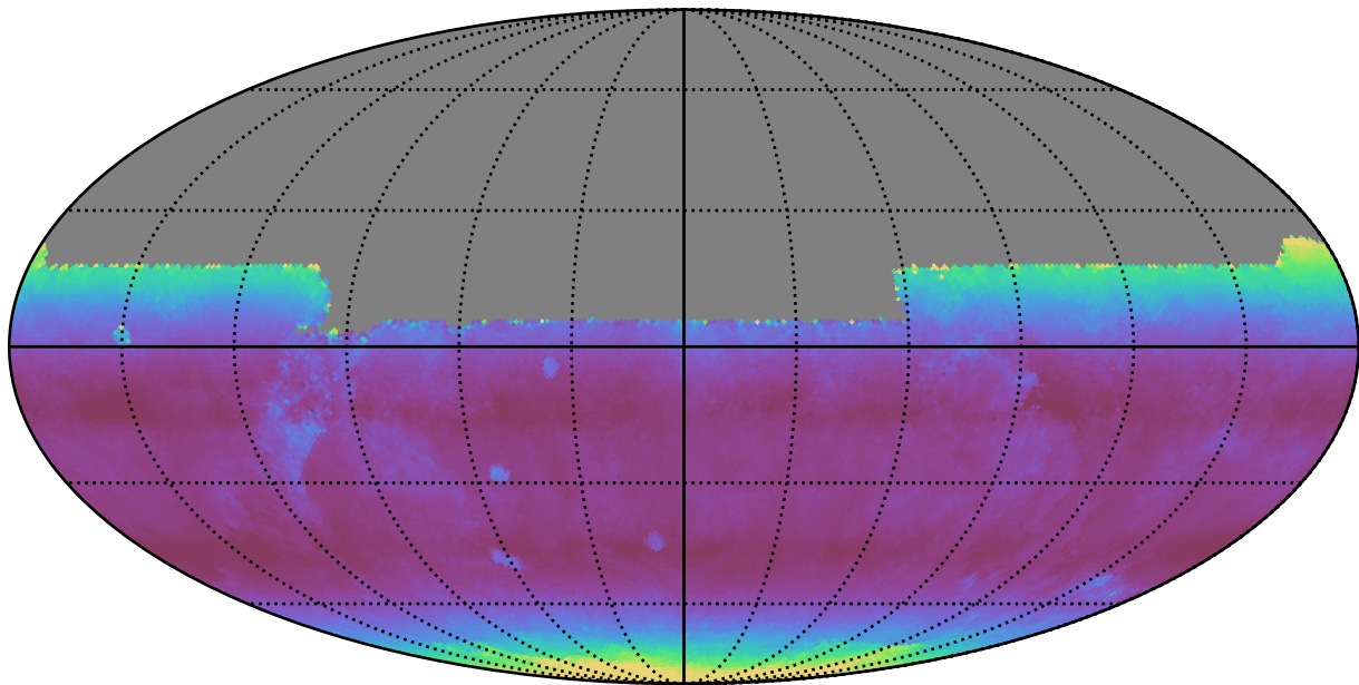
ddf_loaded_fl2_v3.4_10yrs All sky y band: Median airmass
