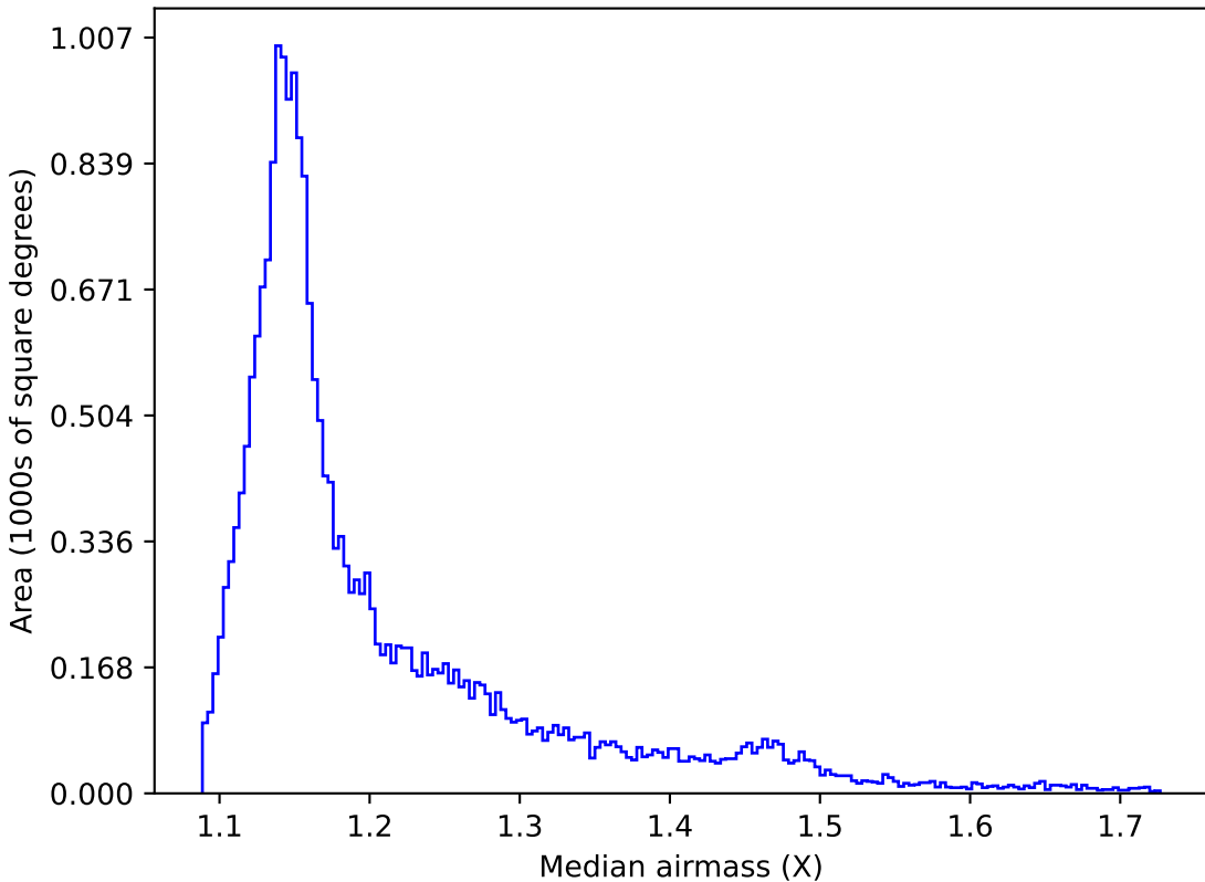
ddf_loaded_fl2_v3.4_10yrs All sky y band: Median airmass
