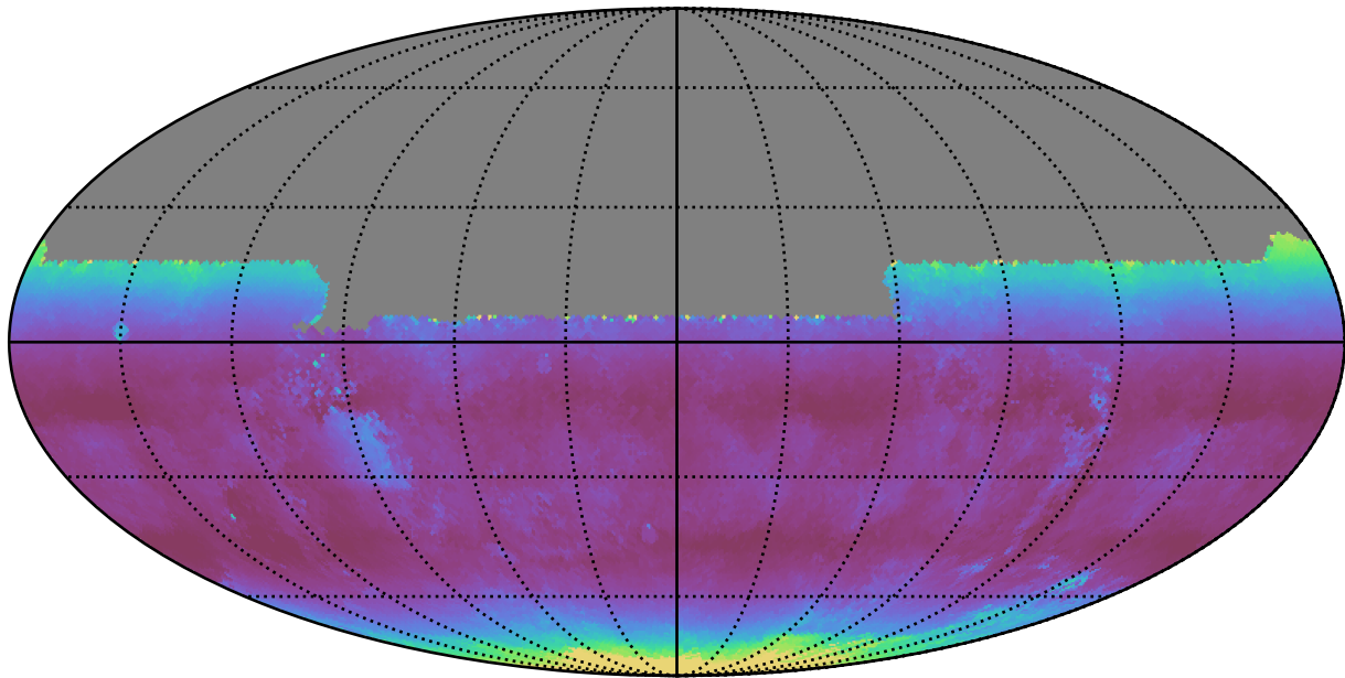
ddf_loaded_fl2_v3.4_10yrs All sky u band: Median airmass
