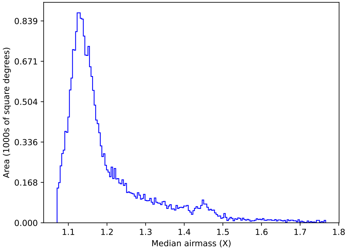
ddf_loaded_fl2_v3.4_10yrs All sky u band: Median airmass
