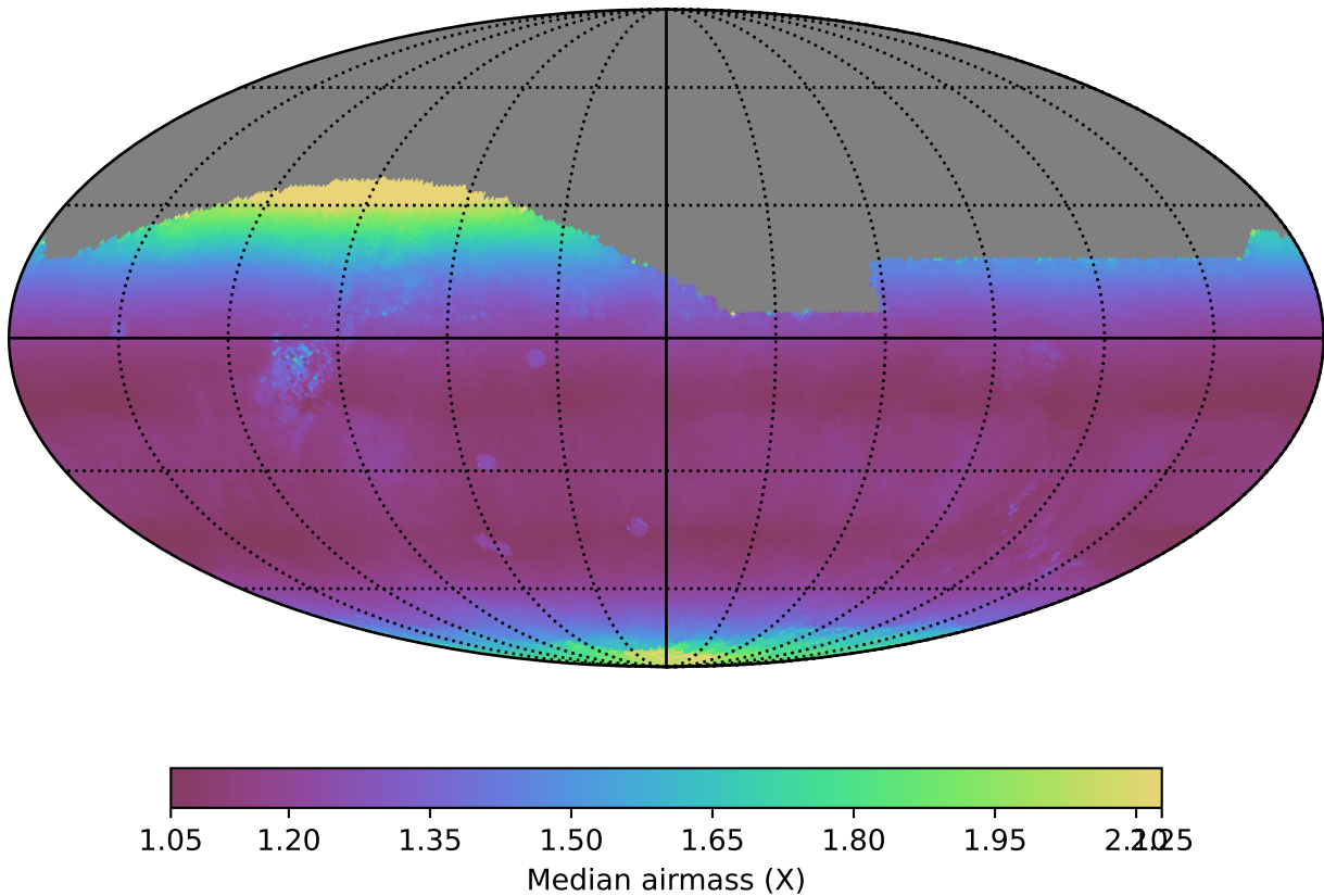
ddf_loaded_fl2_v3.4_10yrs All sky r band: Median airmass
