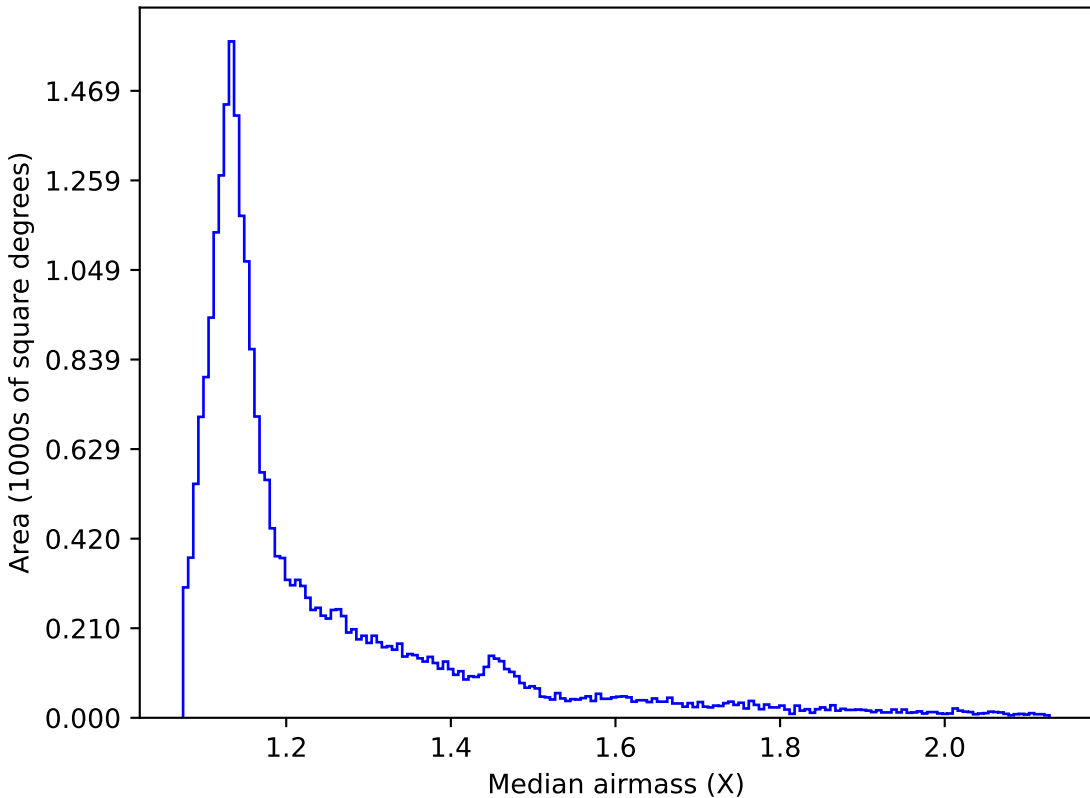
ddf_loaded_fl2_v3.4_10yrs All sky r band: Median airmass
