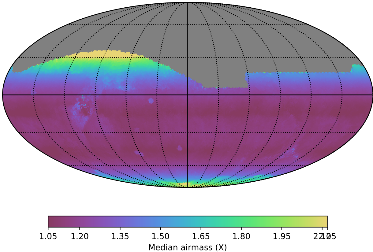
ddf_loaded_fl2_v3.4_10yrs All sky i band: Median airmass
