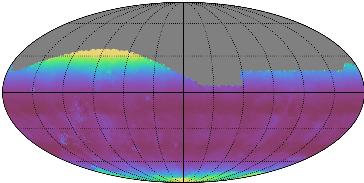
ddf_loaded_fl2_v3.4_10yrs All sky g band: Median airmass
