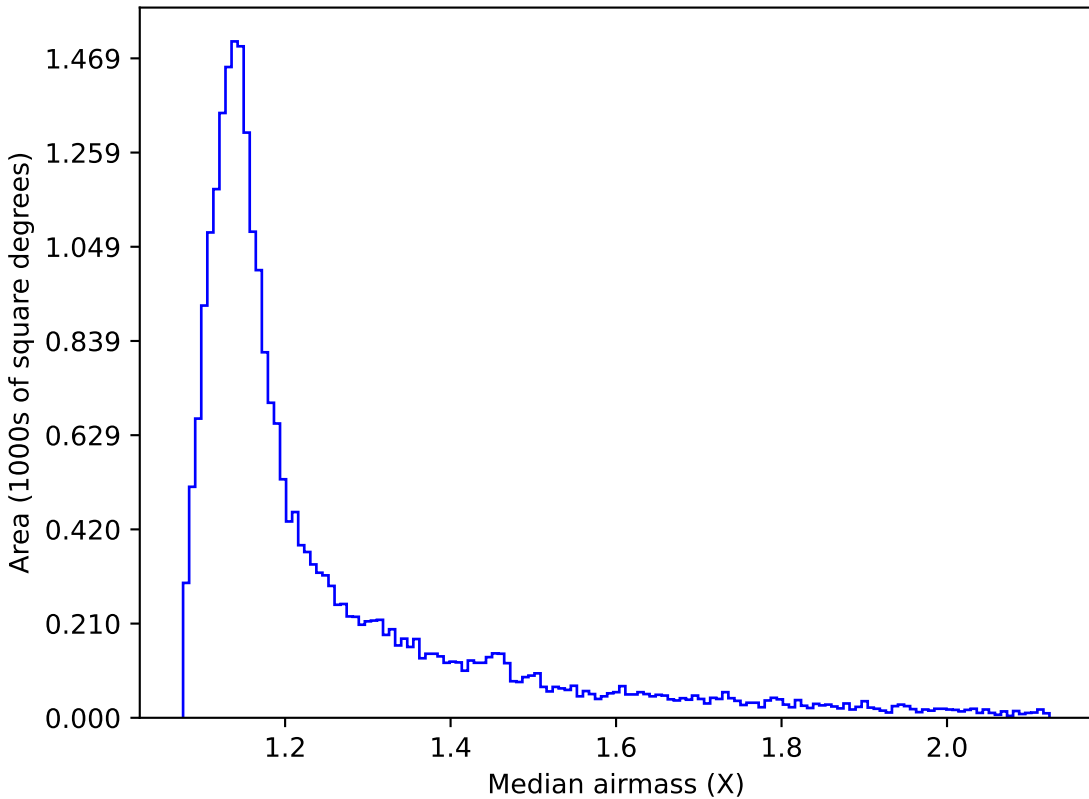
ddf_loaded_fl2_v3.4_10yrs All sky g band: Median airmass
