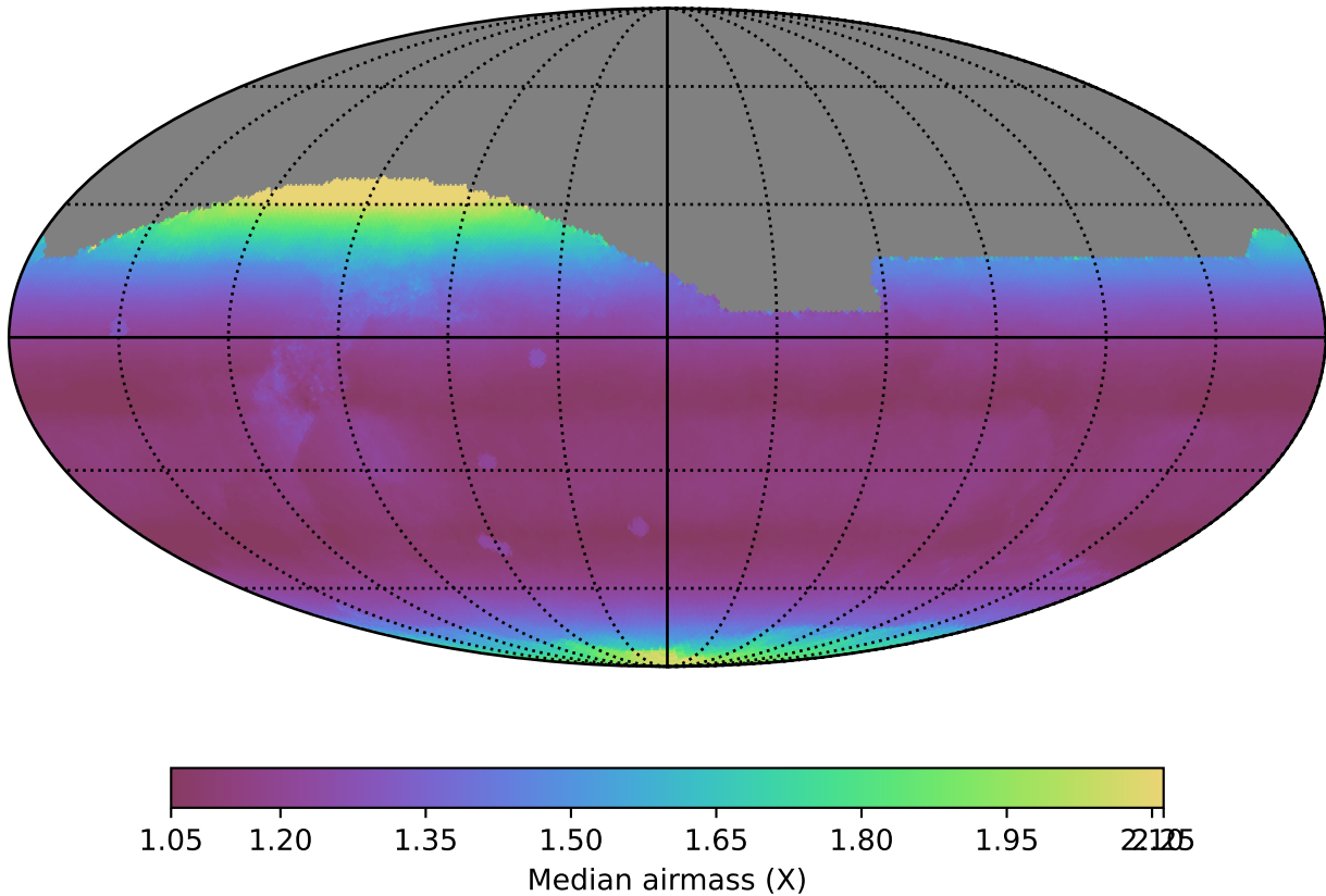
ddf_loaded_fl2_v3.4_10yrs All sky all bands: Median airmass
