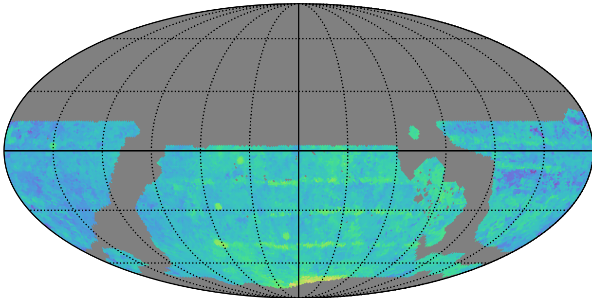
ddf_loaded_fl2_v3.4_10yrs WFD z band: Median Season Length
