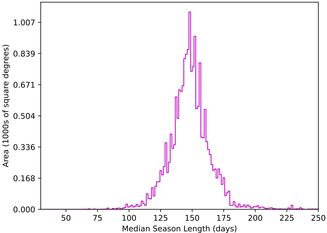
ddf_loaded_fl2_v3.4_10yrs WFD z band: Median Season Length
