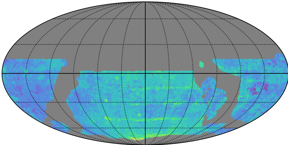
ddf_loaded_fl2_v3.4_10yrs WFD y band: Median Season Length
