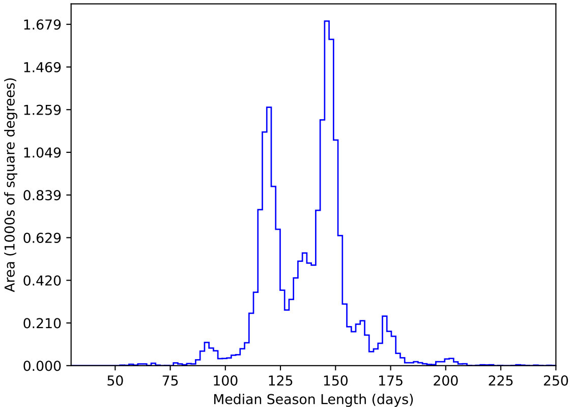
ddf_loaded_fl2_v3.4_10yrs WFD y band: Median Season Length
