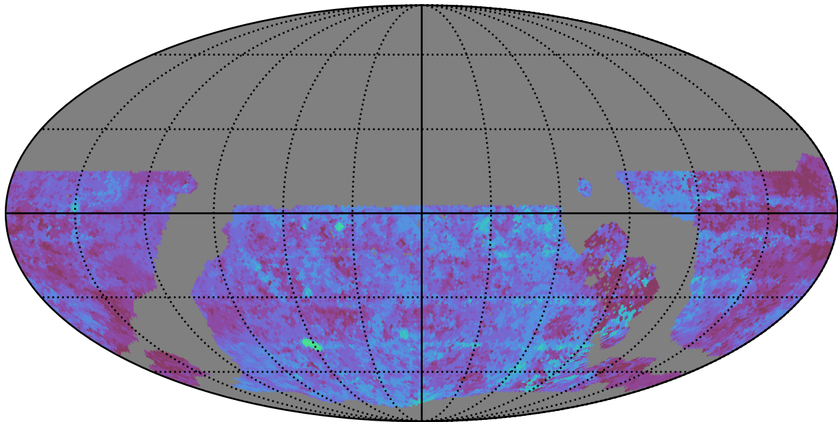
ddf_loaded_fl2_v3.4_10yrs WFD u band: Median Season Length
