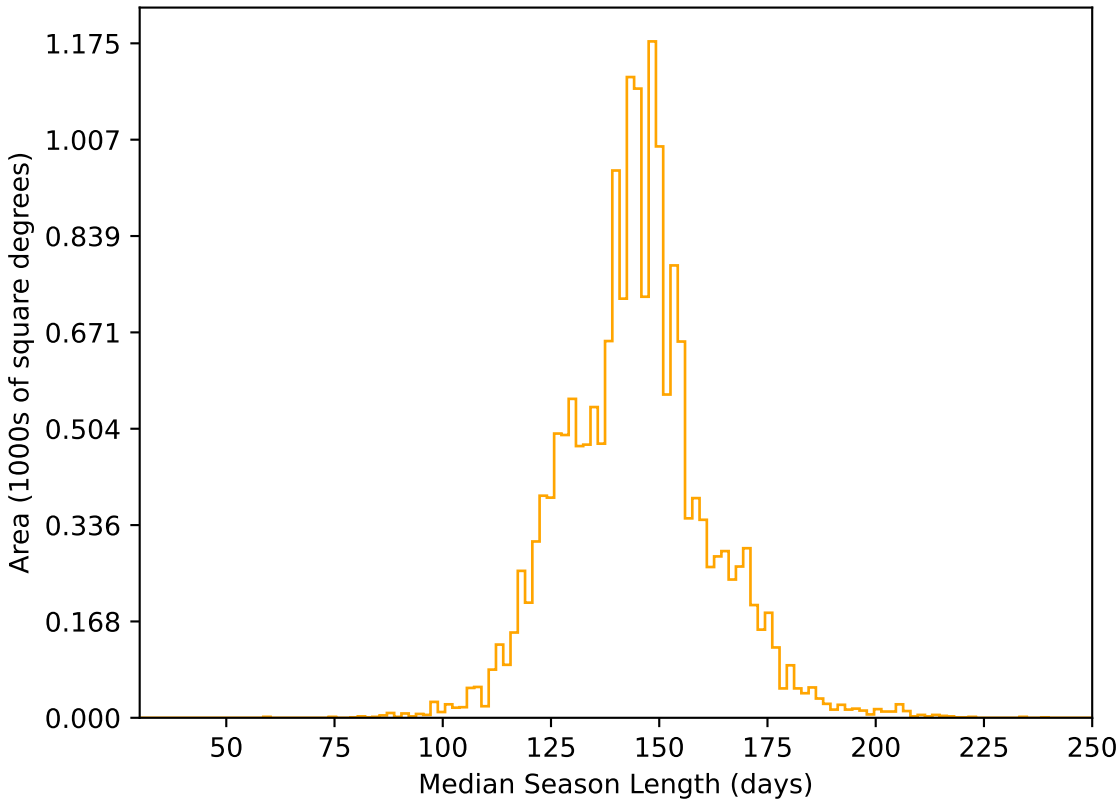
ddf_loaded_fl2_v3.4_10yrs WFD r band: Median Season Length
