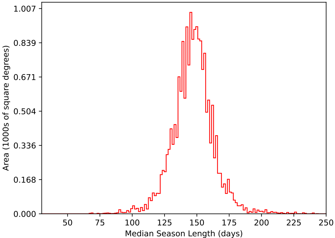
ddf_loaded_fl2_v3.4_10yrs WFD i band: Median Season Length
