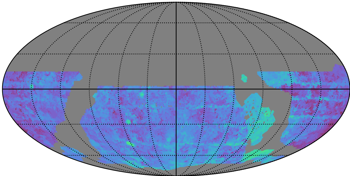
ddf_loaded_fl2_v3.4_10yrs WFD g band: Median Season Length
