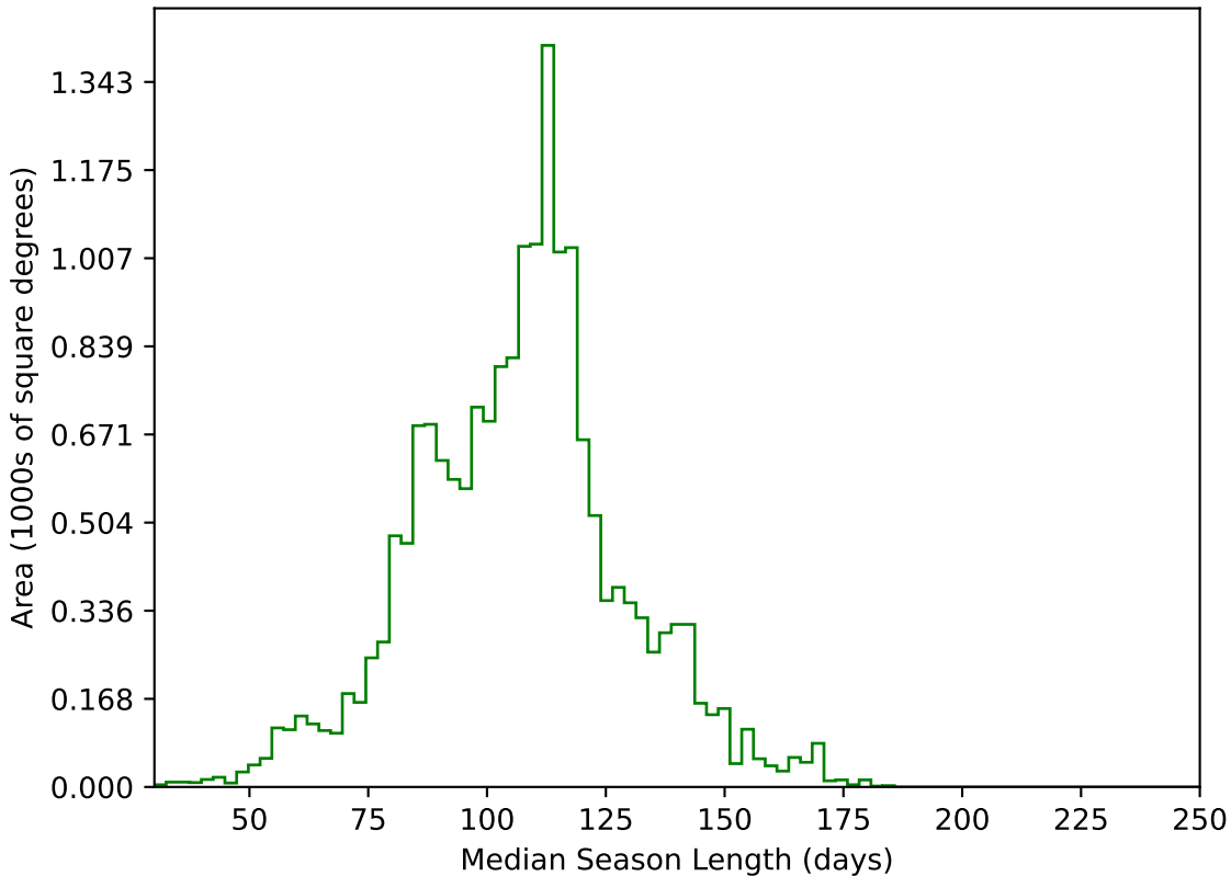
ddf_loaded_fl2_v3.4_10yrs WFD g band: Median Season Length
