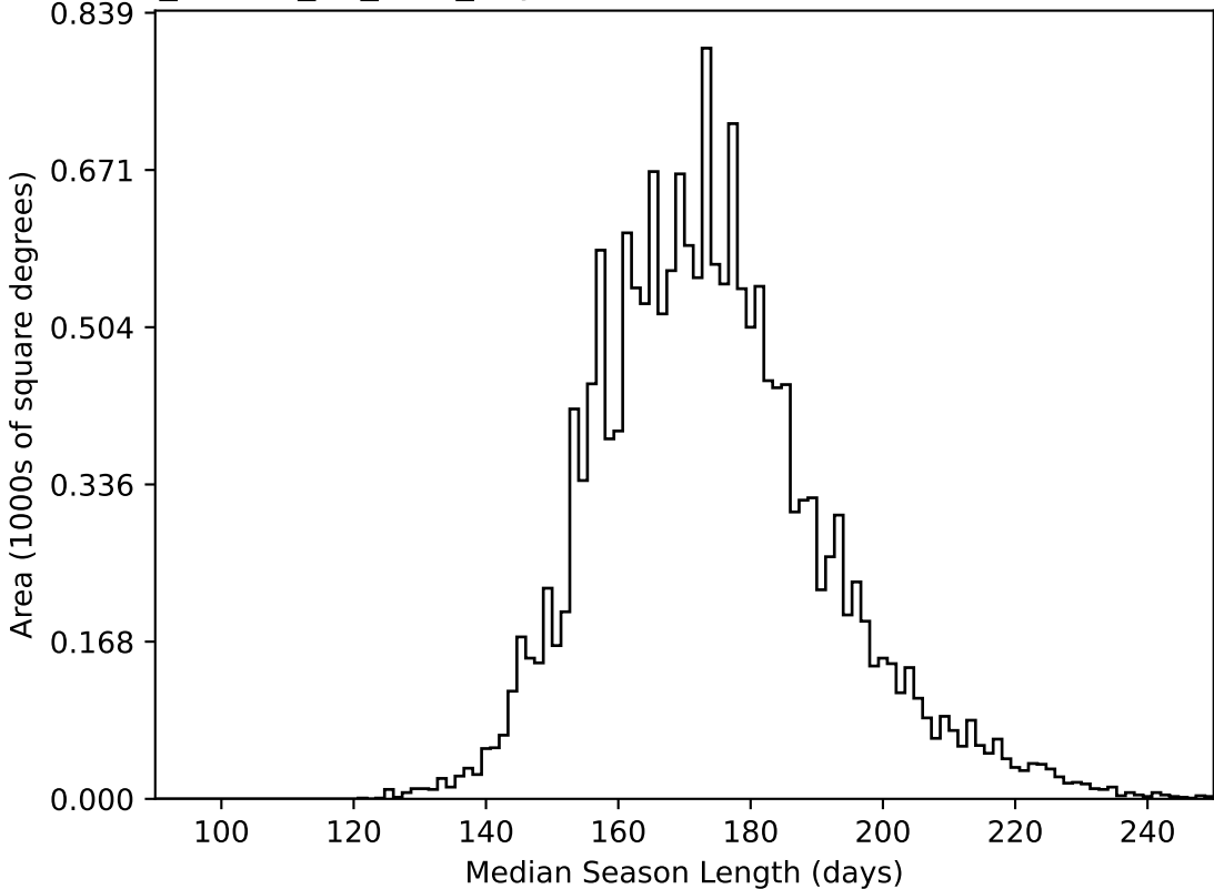
ddf_loaded_fl2_v3.4_10yrs WFD all bands: Median Season Length
